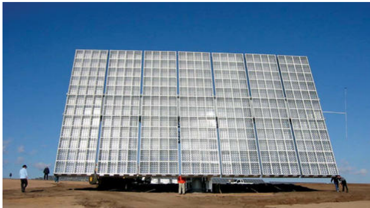
Figure A-7 Amonix: Flat Acrylic Lens Concentrator with Silicon Cells (Source: NREL)
